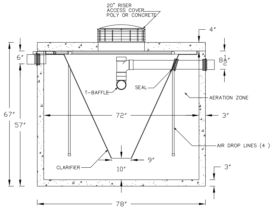
SIDE VIEW CUTAWAY TO SHOW INTERNAL DETAILS
