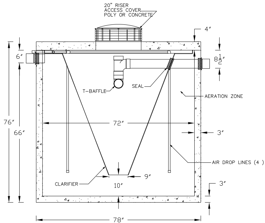
SIDE VIEW CUTAWAY TO SHOW INTERNAL DETAILS
