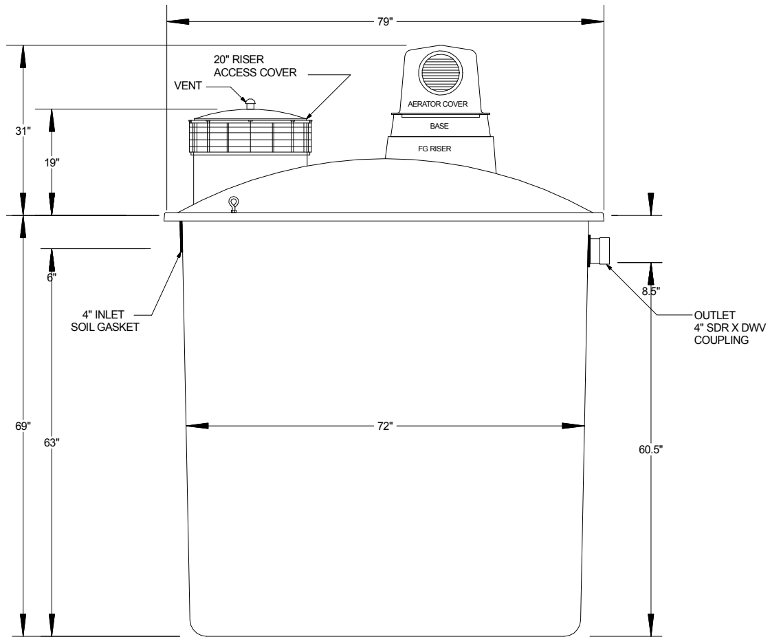
SIDE VIEW
